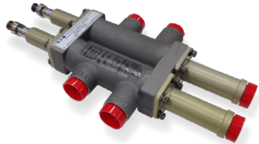
3000 psi Brake Metering Valve
